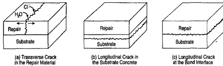
Figure 10. Types of failures in repaired systems (19)
