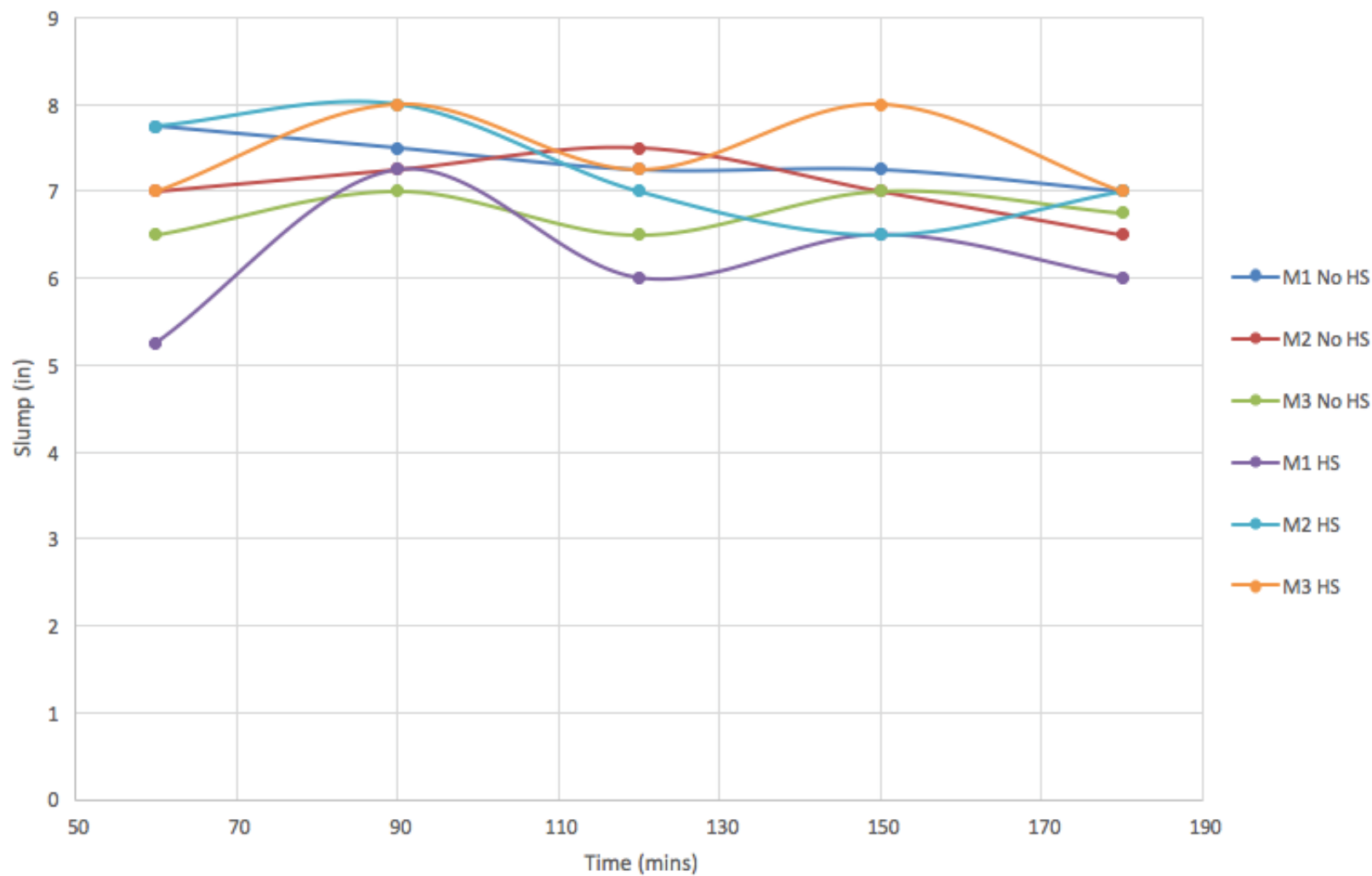
Slump - Moderate Weather
