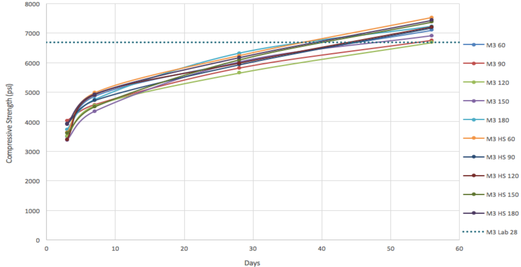
M3 - Compressive strength vs age - MODERATE Weather
