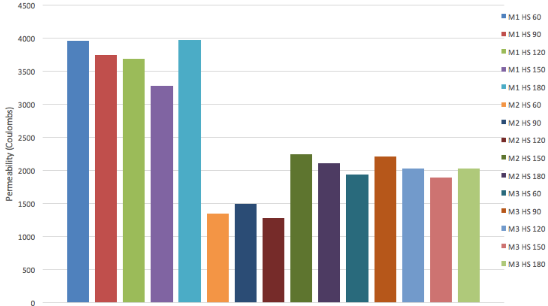
Permeability at 90 days - with HS - MODERATE Weather
