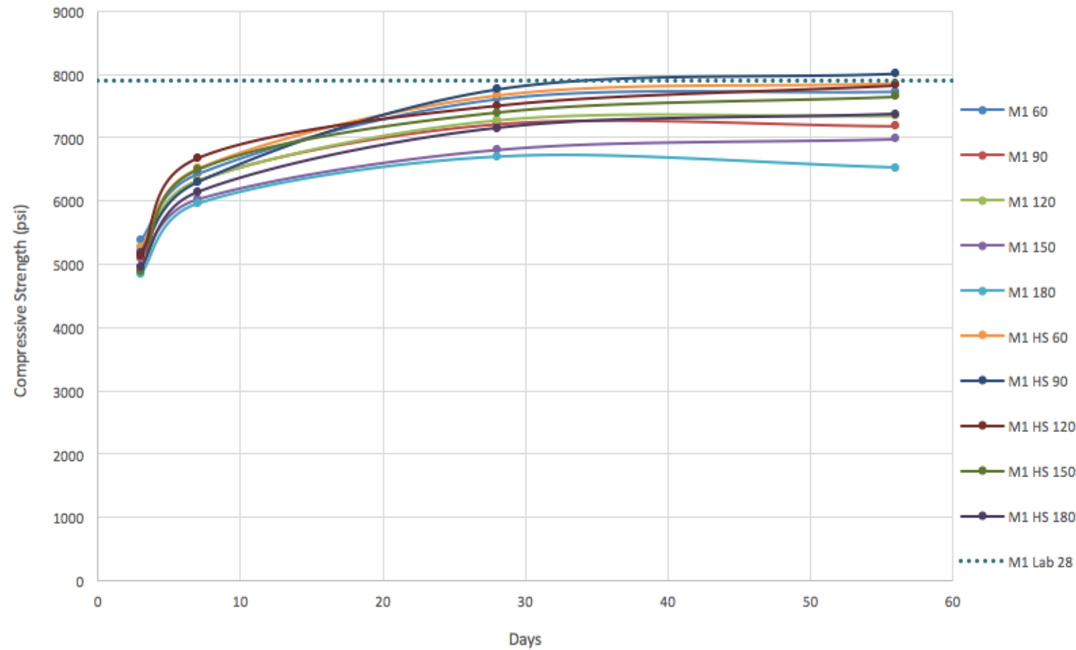
M1 - Compressive strength vs age - MODERATE Weather
