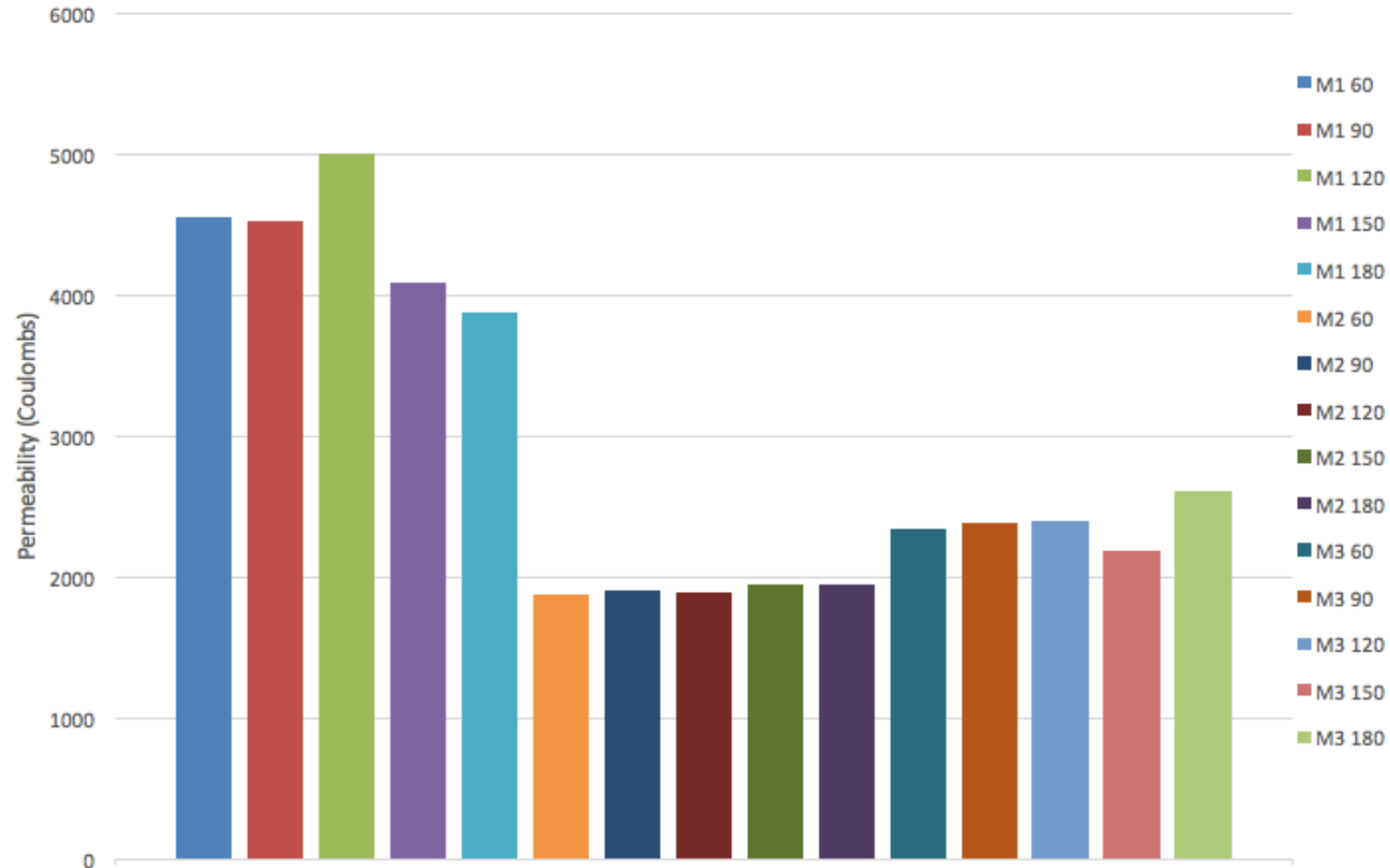
Permeability at 90 days - NO HS - MODERATE Weather
